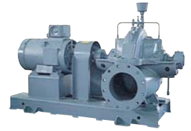
DV type both-side suction centrifugal pump For waterworks and factories φ200~φ350, 11kW~250kW
