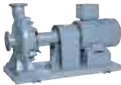
HOV type end suction centrifugal pump For air conditioning (Especially high forced pressure application) φ65~φ250, 0.75kW~160kW
