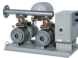
Neuro Junior Water Ace for water supply in buildings and apartment house φ40~φ65, 0.75kW~5.5kW
